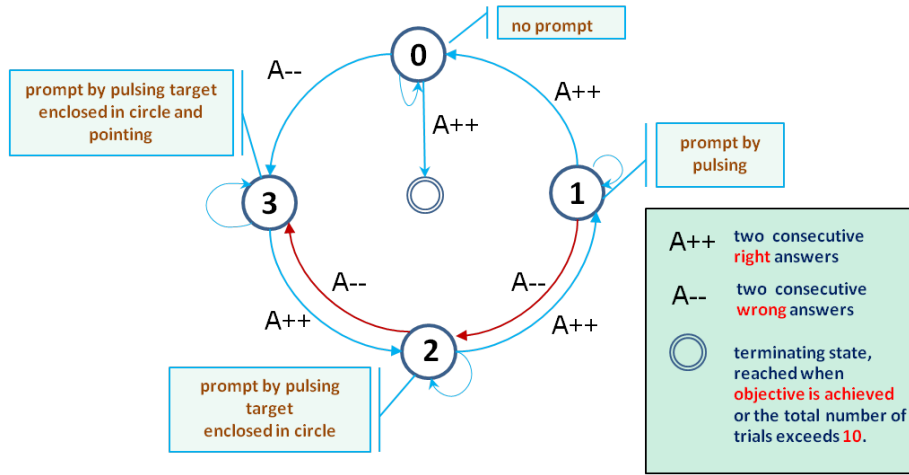
Figure 3. Finite state machine for prompt adaptation. It emits two types of symbols: A++ for two consecutive right answers, and A-- for two consecutive wrong answers. The degree of prompting is increased or decreased based on a child’s performance. iPad tasks begin in State 3; NET tasks begin in State 0. Not shown here is the trial count, which forces a transition to the terminating state when it exceeds 10.
