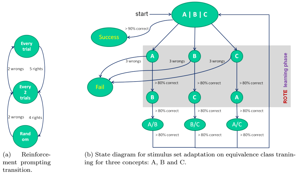
Figure 2. State transition diagram for reinforcement prompting and stimulus set adaptation.
