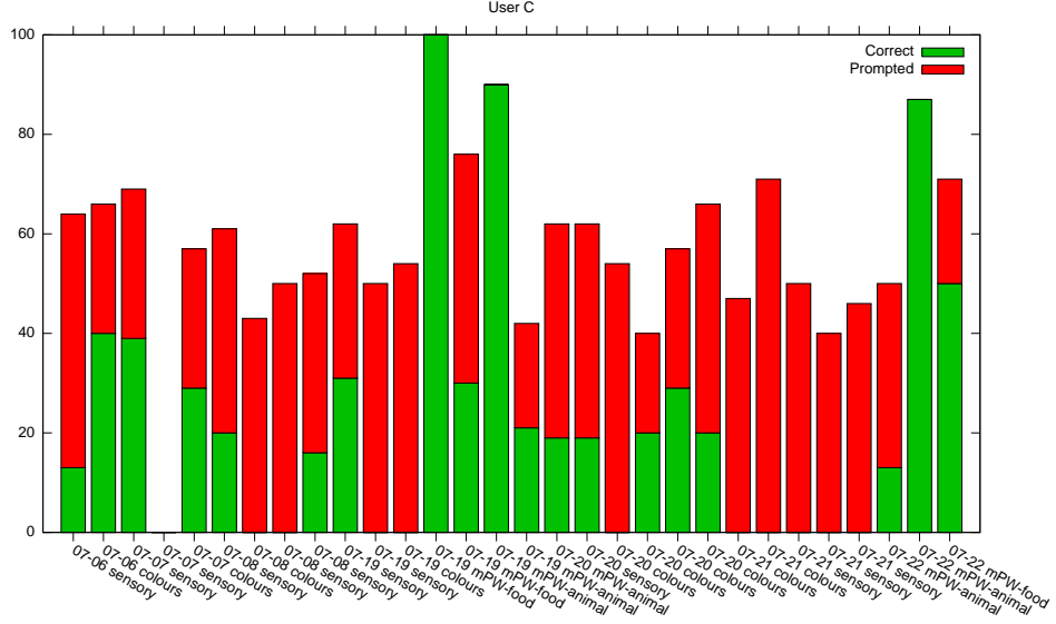
Figure 15. Results for subject C, showing difficulty with simpler receptive matching tasks.
