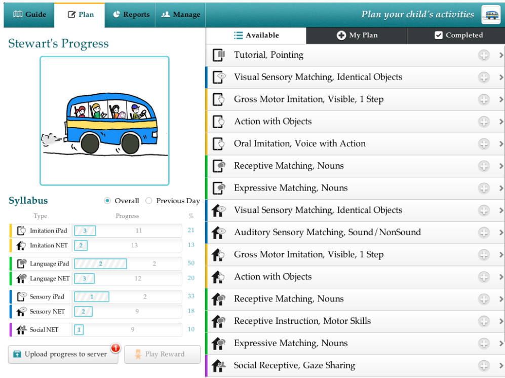
Figure 4. Screenshot of Playpad’s daily schedule. Left of screen includes details of the current child’s profile and progress; Right of screen lists tasks that Playpad has made available.
